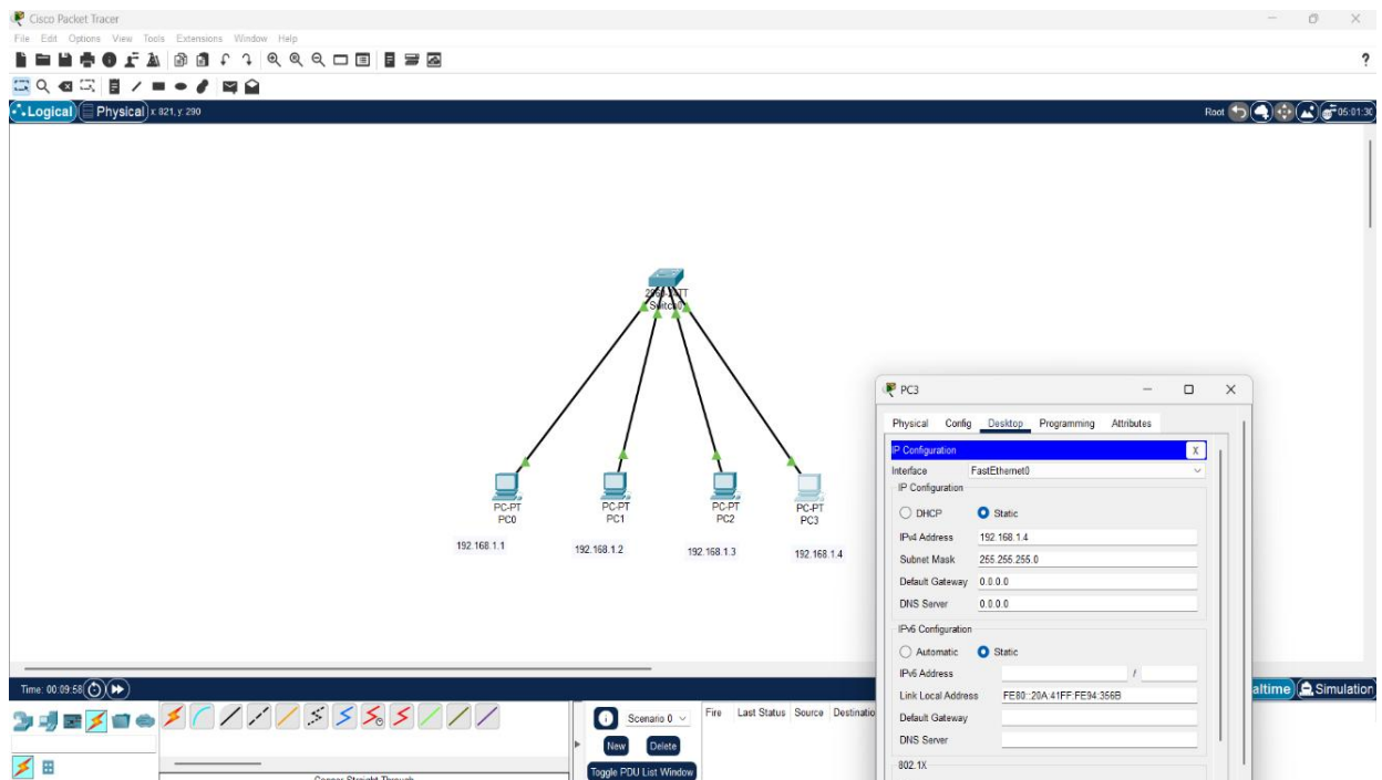
Figure 2.4: Assigning IP Addresses
